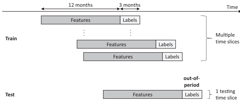
Fig. 4. Time slices for multi-slicing (adapted from Gattermann-Itschert and Thonemann (2021)).
