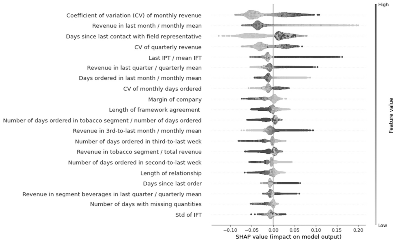
Fig. 9. SHAP summary plot to evaluate global importance of features.
