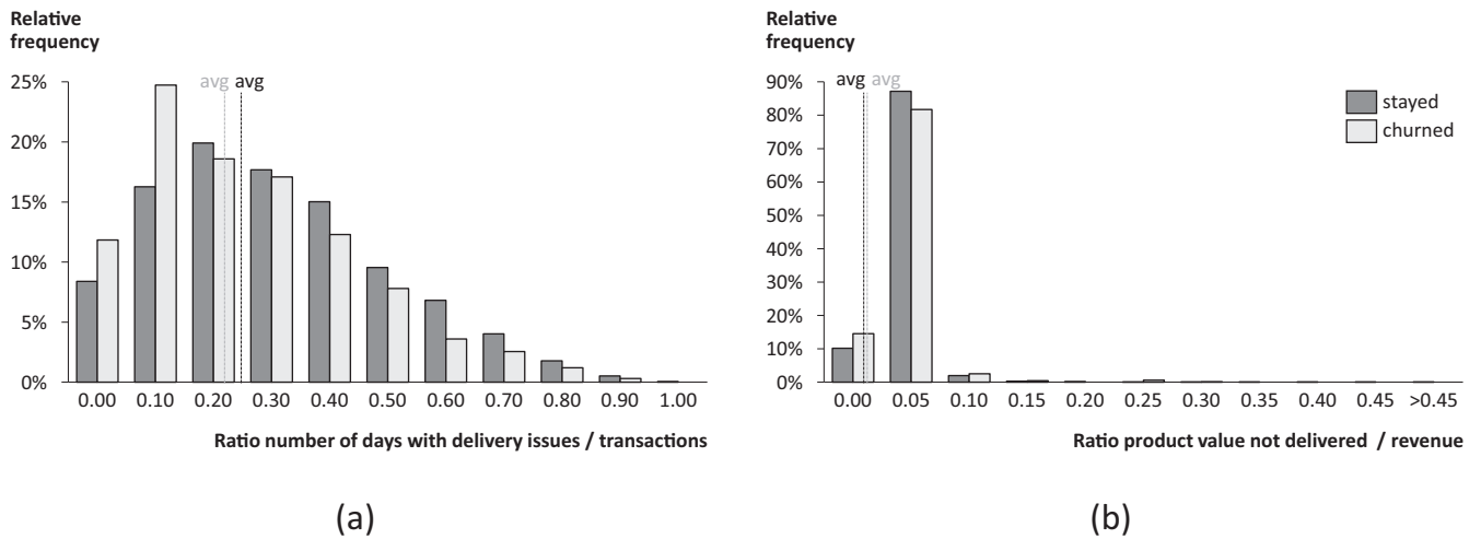
Fig. 6. Histogram of relative frequency for delivery performance features (stayed/churned).
