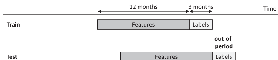
Fig. 3. Training and testing time slices for out-of-period testing.
